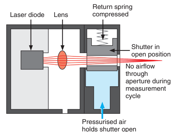
Figure 3c - Shutter is held open by pressurised air, whilst air bleed/blast is shut off to eliminate air turbulence along the laser beam
