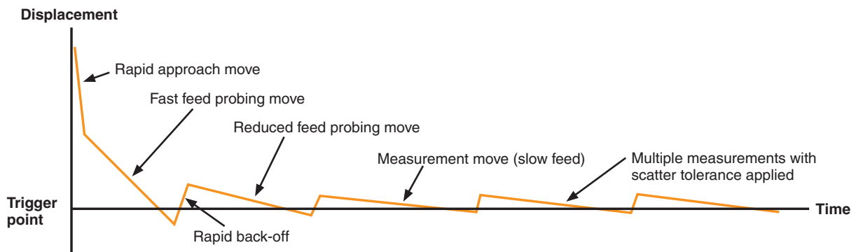
Figure 7 - Multiple measurement moves are designed to ensure that residue on the tool does not affect the measurement result
