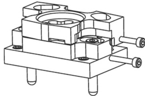
Figure 11 - 3-plate adjuster pack
