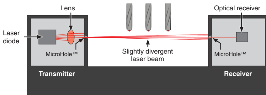
Figure 2 - Renishaw's transmitter unit features a lens that provides a narrow laser beam that passes through a small MicroHole™. The receiver further filters this light using a second MicroHole™, forming a very narrow, parallel measurement laser beam
