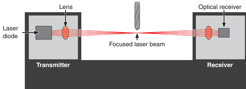
Figure 1 - Transmitter unit of a first generation laser tool setter providing a beam that is focused at a particular point between transmitter and receiver
