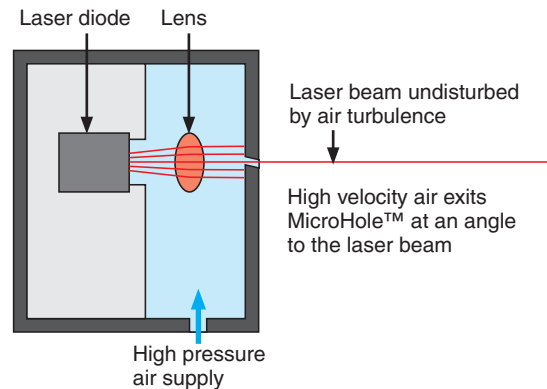
Figure 4 - Renishaw MicroHole™ technology provides continuous protection with no moving parts, even during measurement
