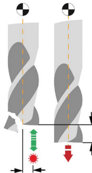
Figure 10 - Edge checking/insert missing detection routine
