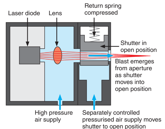
Figure 3b - Shutter is moved to open position by pressurised air, resulting in an air blast through the aperture as the trapped air in the optics chamber escapes
