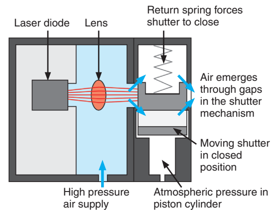
Figure 3a - During machining, conventional laser tool setters are protected by a moving shutter and continuous air 'bleed'
