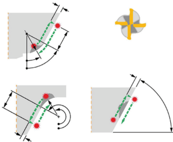
Figure 9 - Profile checking routines
