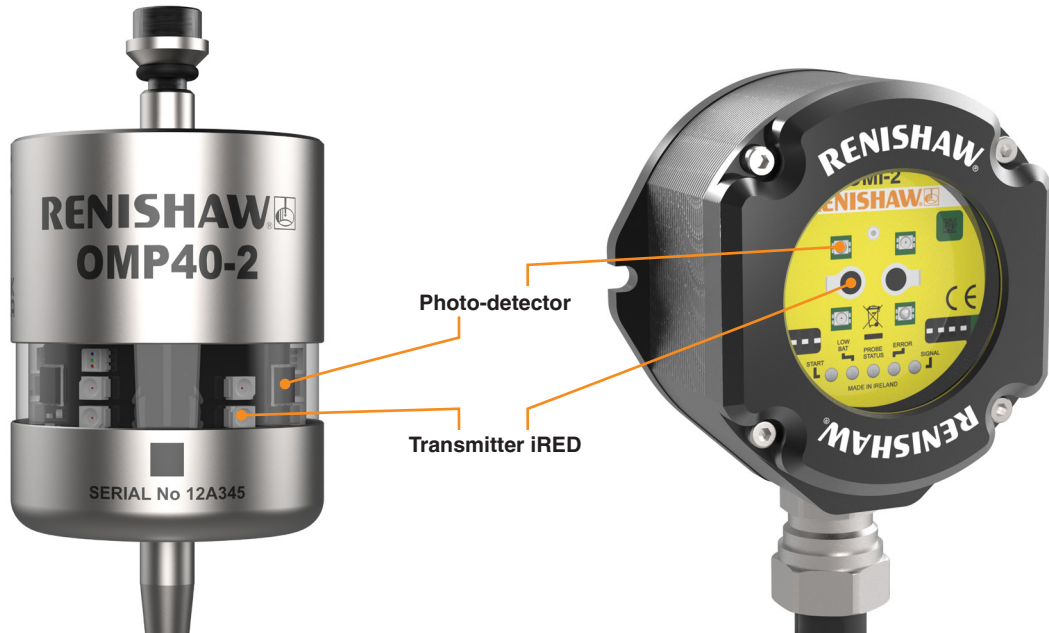
Figure 1: OMP40-2 workpiece inspection probe with optical transmission
