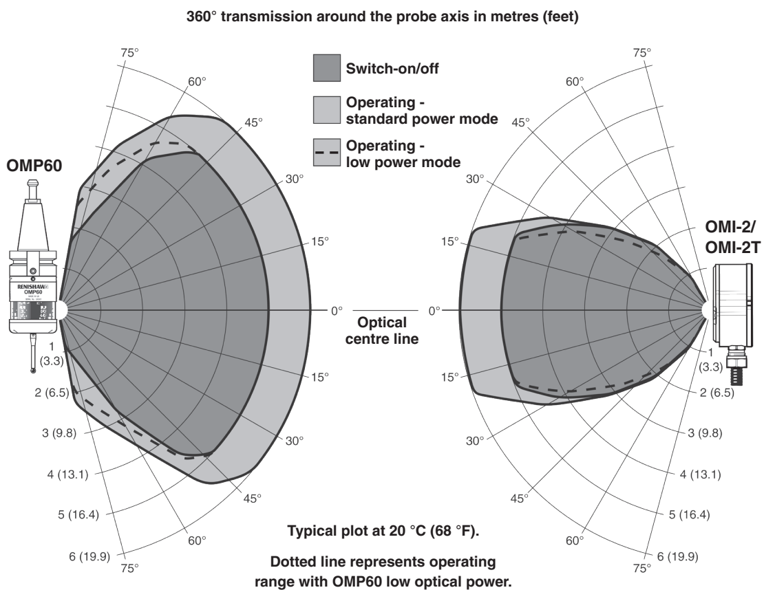
Figure 4: transmission plots of an OMP60 probe and OMI-2/OMI-2T interfaces
