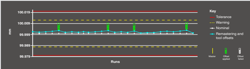
Process Monitor run chart showing CNC updates
