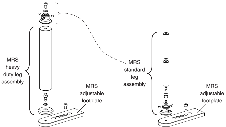
Assembly with MRS heavy duty leg
